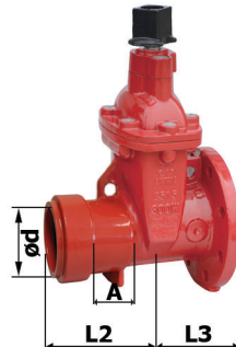
MECHANICAL JOINT (MJ)
