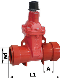
SLIP X SLIP (SS)
