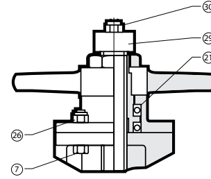
FIG. 84, STAINLESS STEEL - FULL PORT - BI-DIRECTIONAL RESILIENT SEAT
